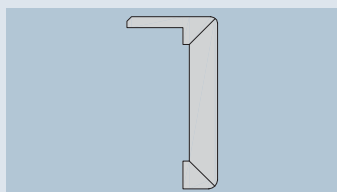
Exclusive architrave 80mm
